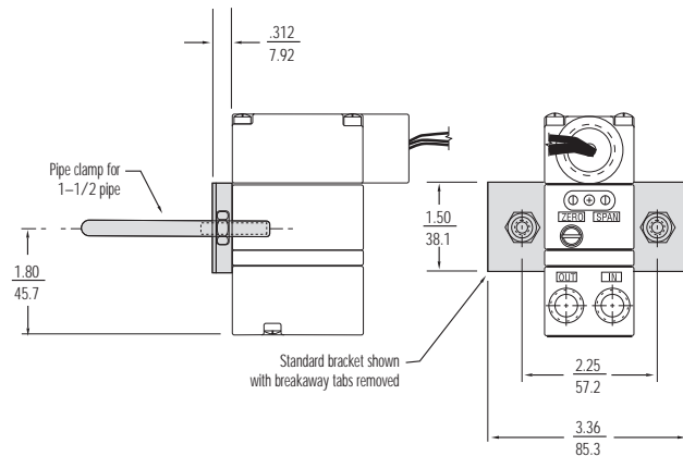
Figure 2 - Standard 1 1/2" Pipe Mount
