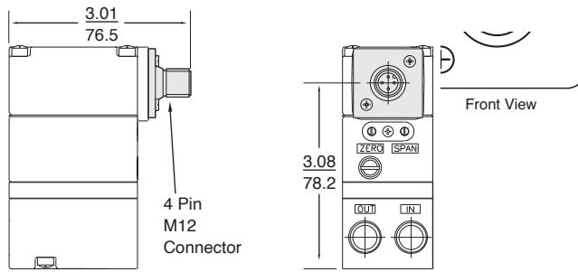
Figure 6 - M12 Connector
