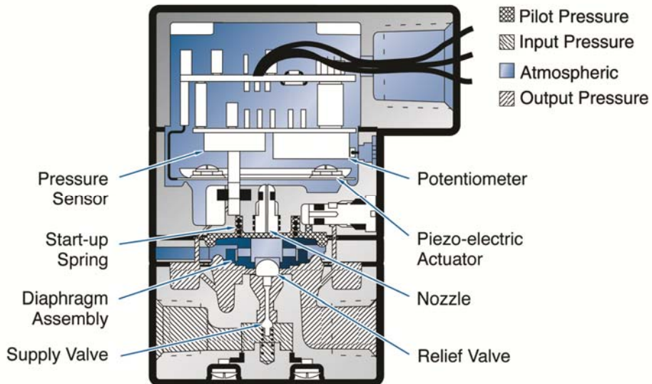
Figure 2 – ControlAir Model 900
