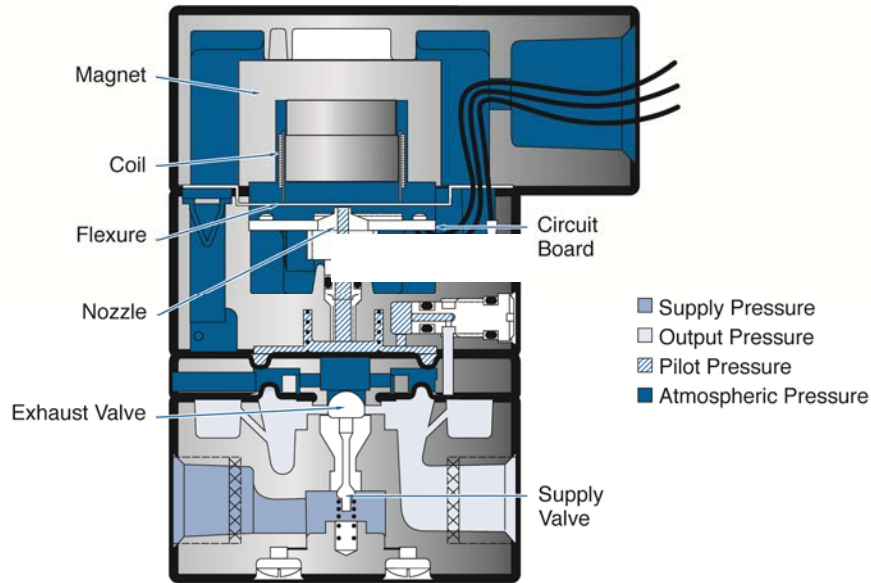
Figure 1 – ControlAir Model 550
